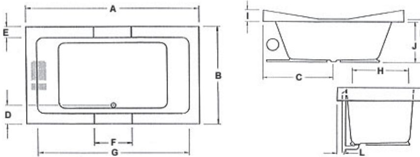
Tub must be set in Mortar Base
